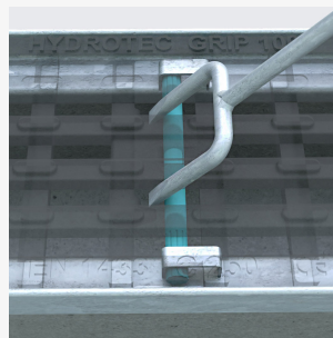
Screwless locking system
